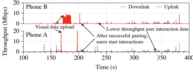
Fig. 9. Another AR app, Just A Line, also exhibit smaller data spikes after the initial large ones, corresponding to users drawing virtual graffiti.
