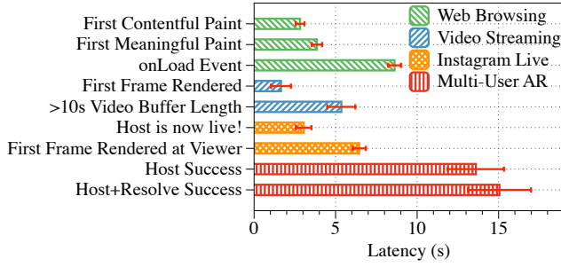
Fig. 4. User-perceived latency
